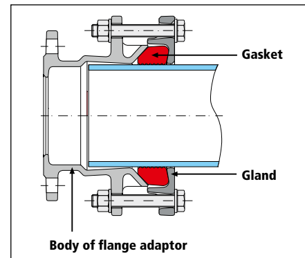
Fig. 10.6: View in section of an assembled wide-tolerance flange adaptor
