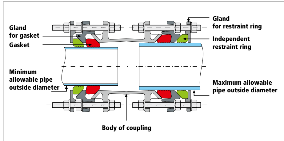
Fig. 10.9: Coupling with mechanical joints and independent restraint system
