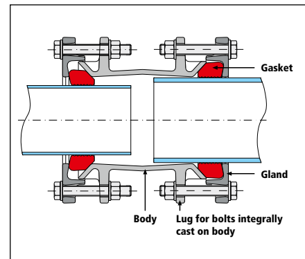
Fig. 10.2: View in section of an assembled wide-tolerance coupling
