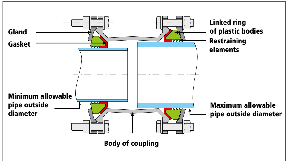
Fig. 10.8: Coupling with mechanical joints and integrated restraint system (double bolts)
